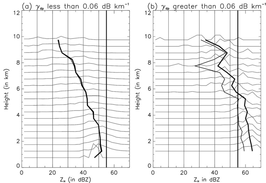
FIG. 9. Mean vertical profiles of reflectivity ( Z_H ) in two contrasted cases: (a) \gamma_{DP} < 0.06 \text{ dB } ^\circ\text{km}^{-1} and (b) \gamma_{DP} > 0.06 \text{ dB } ^\circ\text{km}^{-1} . The histogram of Z_H for each height level between 1 and 10 km MSL is plotted. The vertical thick line corresponds to Z_H = 55 \text{ dBZ} .
